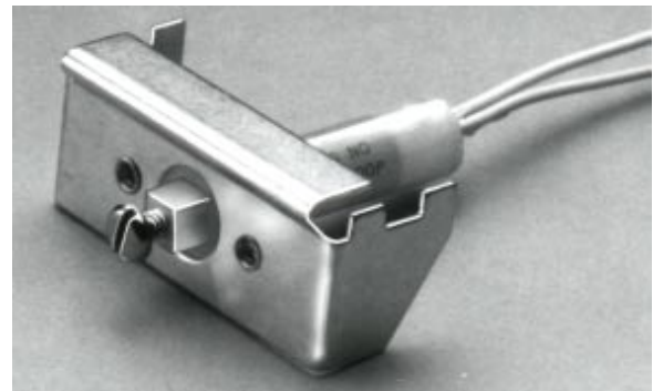
TSC-20 Clip Mounting
